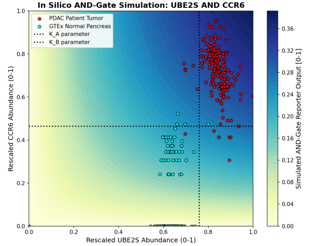
Fig. 4: 2D Contour heatmap demonstrating simulation output of UBE2S AND CCR6 logical AND gate, with rescaled expression and tumor/normal sample overlays.
