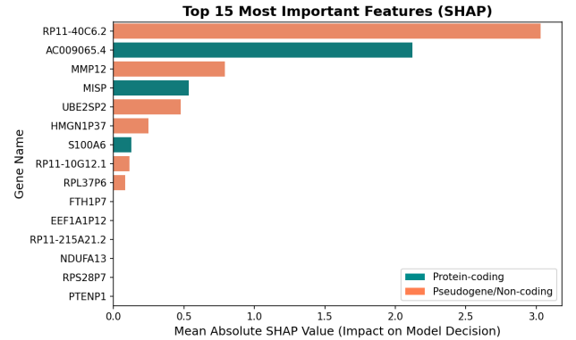
Fig. 2: SHAP summary plot showing feature importances for the top-ranked genes driving the L1 Logistic Regression classifier.
