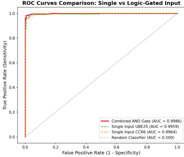
Fig. 5: ROC curves comparing individual inputs (UBE2S, CCR6) against the combined logic gate output.
