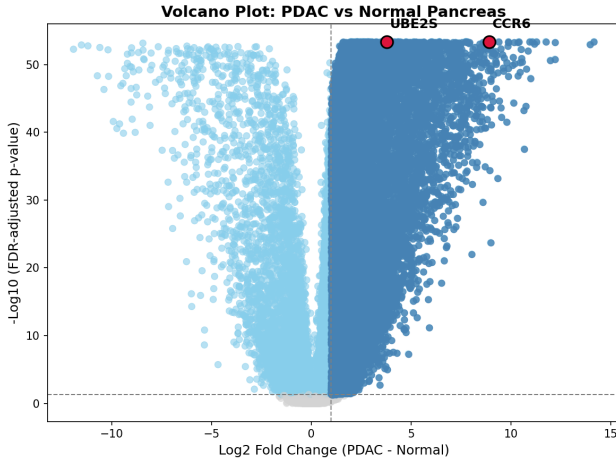
Fig. 1: Volcano plot highlighting significantly differentially expressed genes in the discovery cohort (TCGA-PAAD vs GTEx Normal Pancreas). UBE2S and CCR6 are annotated as significant upregulated candidates.
